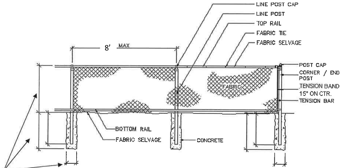
4' - 6' CHAIN LINK FENCE W/ TOP & BOTTOM RAIL
